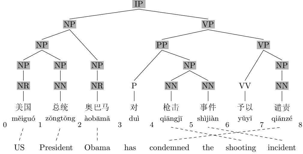
Figure 2: A training example. Tree-to-string rules can be extracted from shaded nodes.
