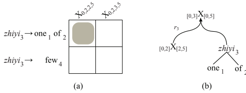
Figure 2: Construct hyperedge from a cube. (a) Cube X_{0,2}zhiyi_3 for source span (0,3). The vertical direction represents the candidate list of zhiyi_3 , while the horizontal direction is a list of nodes that share the same source span (0,2). (b) the hyperedge corresponds to the gray grid in cube (a).
